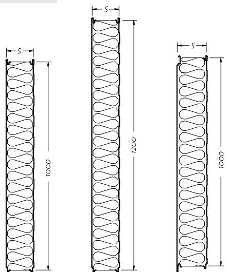
TRIMOTERM STANDARD FTV sirina 1000 mm
